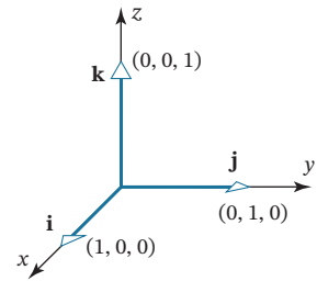
FIGURE 3.5.1 The standard unit vectors.
